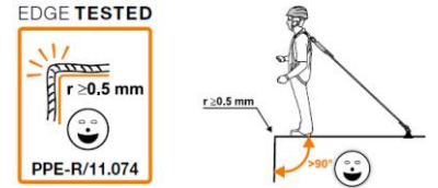
Certified for horizontal use over an edge
