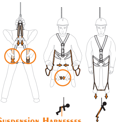
Suspension HARNESSSES Back ATTACHMENT
